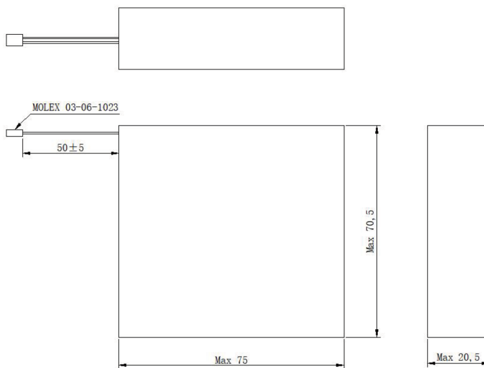
Battery (Unit: mm)
