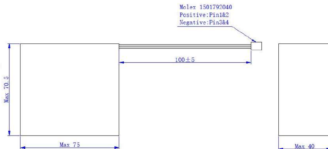
Battery (Unit: mm)
