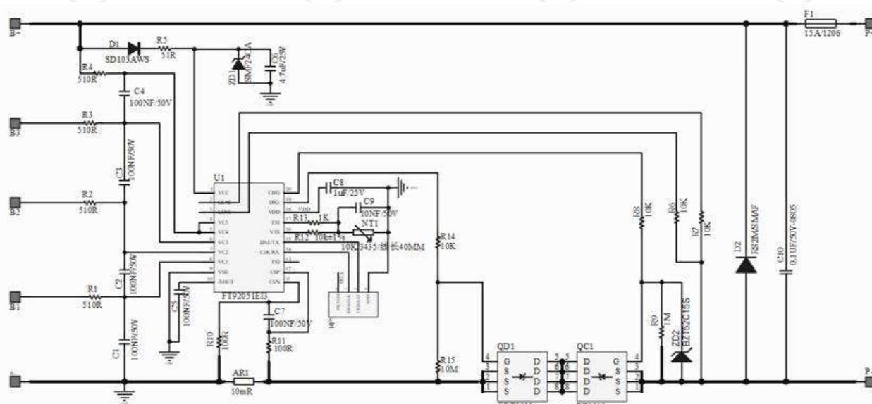
Circuit diagram:
